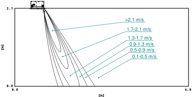
Air velocity distribution (heating) Air flow direction: vertical
