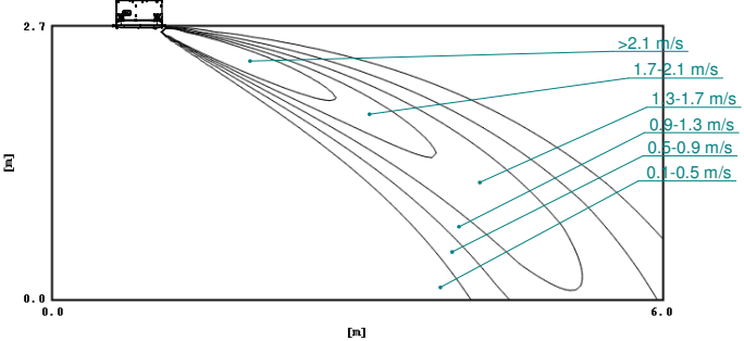
Air velocity distribution (cooling) Air flow direction: horizontal
