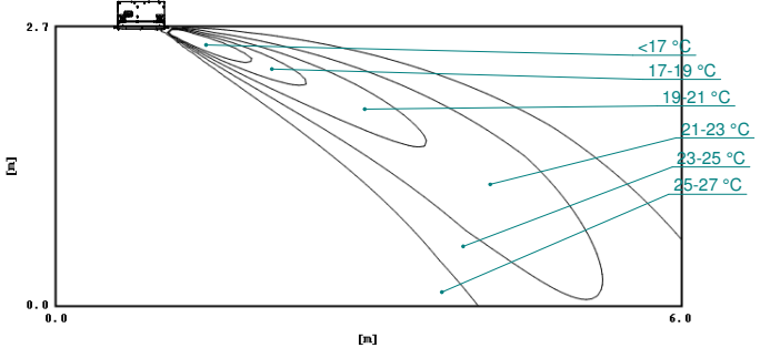
Air temperature distribution (cooling) Air flow direction: horizontal
