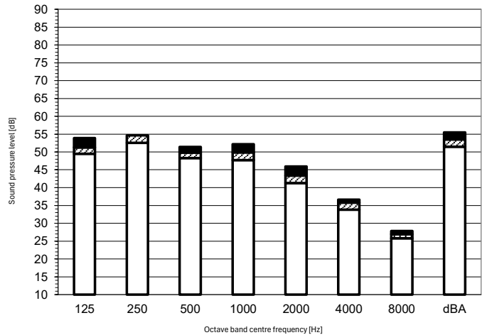
Cooling mode
