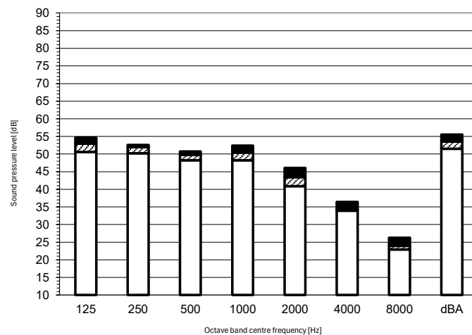
Heating mode
