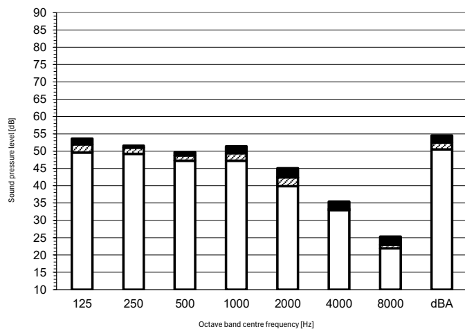
Cooling mode
