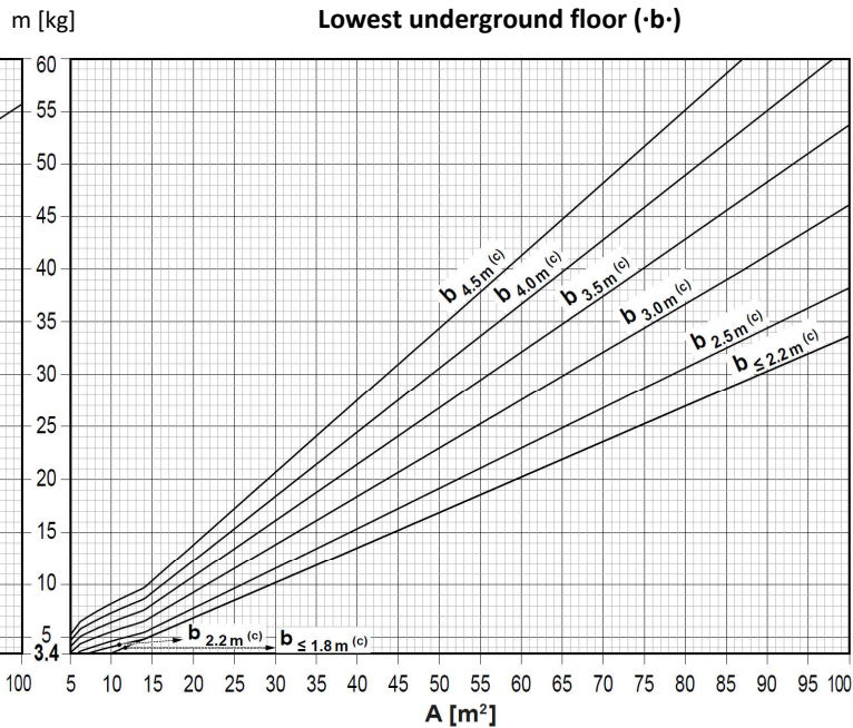
Lowest underground floor (·b·)
