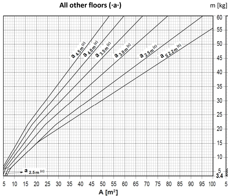
Effective installation height (·c·)
